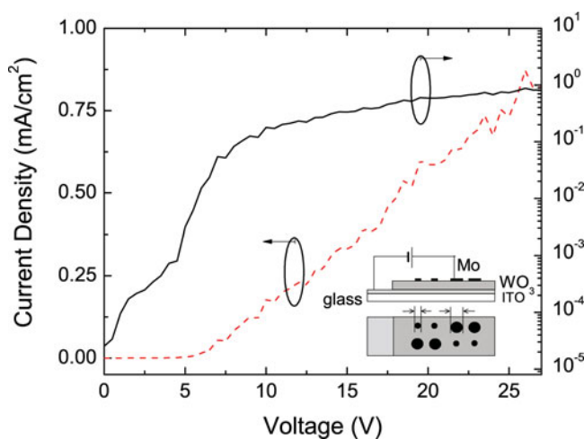
Figure 9. Current density (J)- voltage (V) characteristic of electro-deposited tungsten trioxide film measured by using ITO/WO 3 /Mo structure (as shown in inset).
