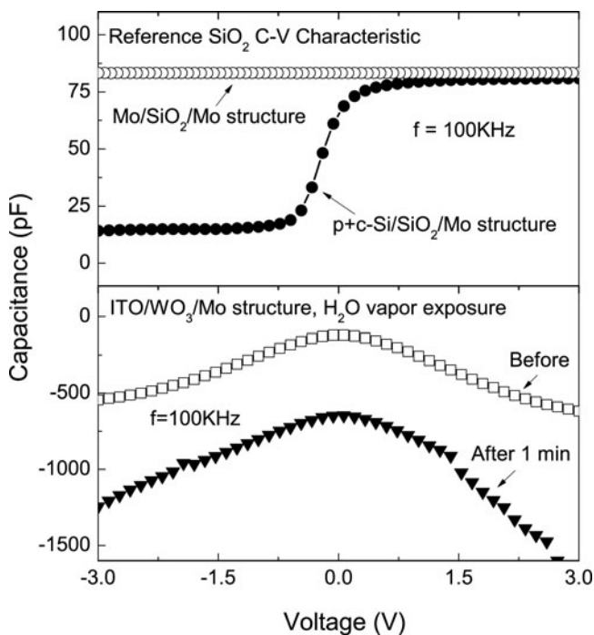
Figure 11. Capacitance (C)- voltage (V) characteristic of: (top) reference PECVD silicon dioxide thin film measured using Mo/SiO 2 /p+c-Si structure and Mo/SiO 2 /Mo structure at 100 kHz; (bottom) as-deposited tungsten oxide thin film and after water vapor exposure for 1 minute measured using Mo/WO 3 /ITO structure at 100 kHz.
