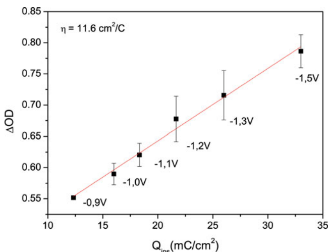
Figure 8. \Delta OD as a function of inserted charge for the WO 3 thin films annealed at 120°C and measured at \lambda = 633 nm for applied potentials of -0.9 to -1.5 V.
