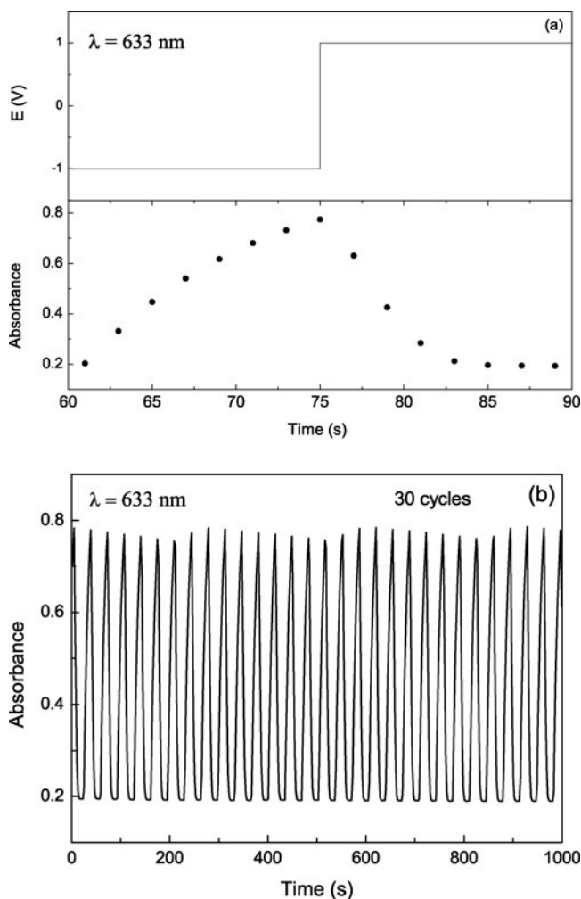
Figure 7. Insertion and extraction cycles of in situ absorbance–time response of \text{WO}_3 film at \lambda = 633 \text{ nm} on the application of potential ( E ) of \pm 1.0 \text{ V} ( 15 \text{ s}/15 \text{ s} ) (a). Last 30 cycles of in situ absorbance–time response of \text{WO}_3 film on the application of potential of \pm 1.0 \text{ V} ( 15 \text{ s}/15 \text{ s} ) for 3,000 cycles (b).
